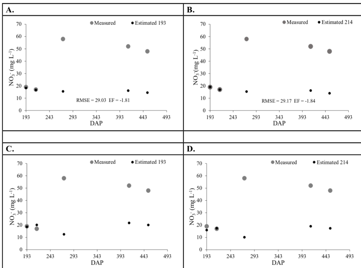
Figure 1. Measured and estimated values of the nitrate concentration in the soil solution from the Vogeler model adapted for 09/23/14 (A) and 10/14/2014 (B) and from the potential model on 09/23/14 (C) and 10/14/2014 (D)
