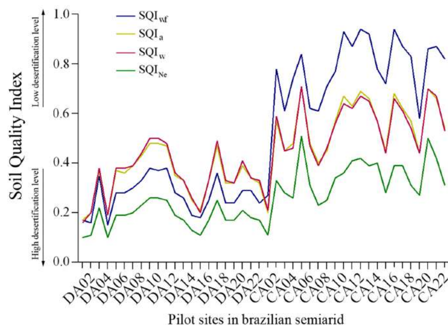
Figure 5. Distribution of the desertification indices (DI) in different pilot sites. DA1 to DA22: desertification area; CA1 to CA22: conservation area; SQI_{wf} : weighted factorial additive soil quality index; SQI_a : additive soil quality index; SQI_w : weighted additive soil quality index; SQI_{Ne} : Nemoro soil quality index.
